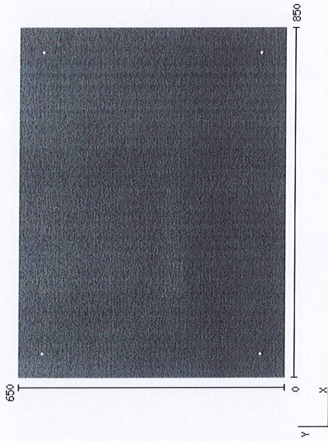
Plaque inox - L 850 x H 650 mm (85 x 65 cm) + 4 TROUS FIXATION (6 mm - 60/60 )
